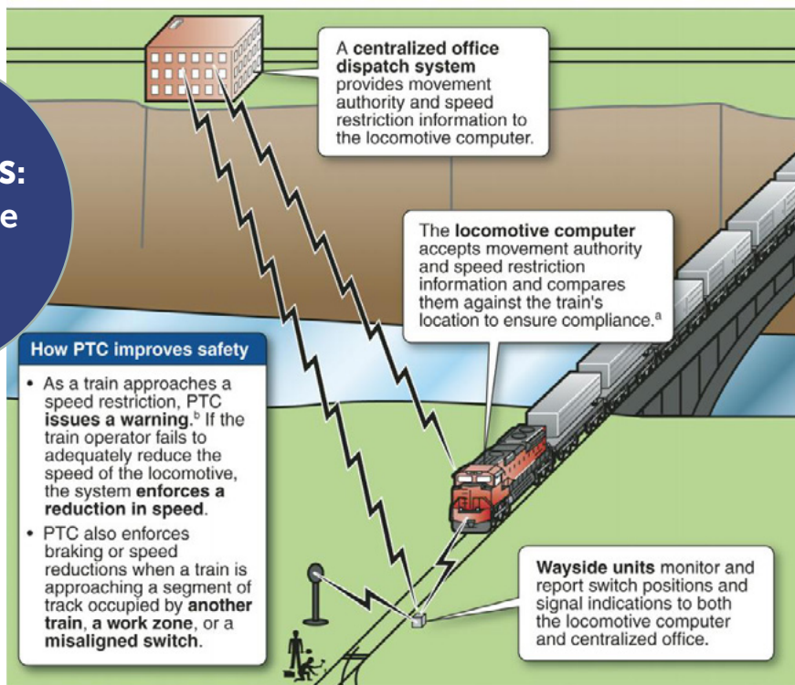
How Positive Train Control works Source: GAO
